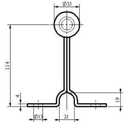
Grande Sliding Gate Stop Bolt-on Over Guide Rail
